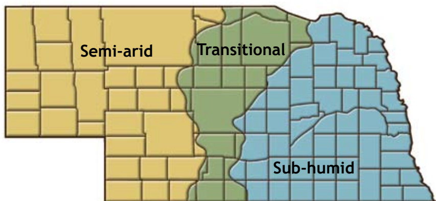
Figure 2. Climatic zones in Nebraska based on weather records from 1961-1990.
