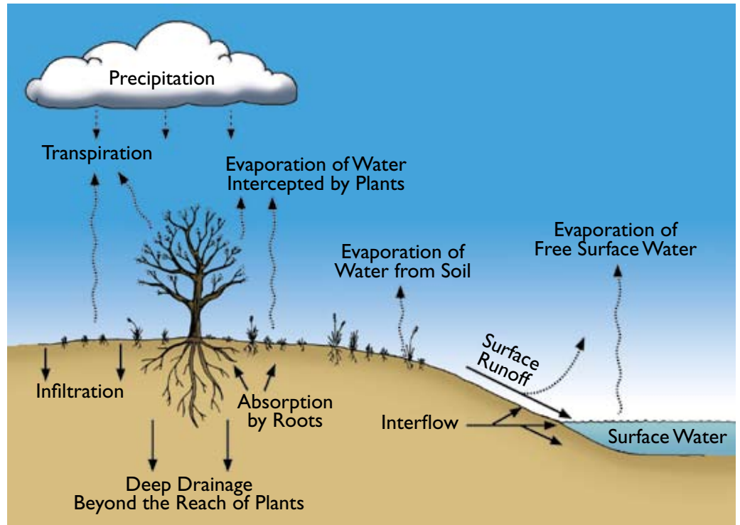
Figure 10. The water cycle showing major processes and pathways of water movement through a watershed. \text{Water inflow} = \text{water outflow} \pm \text{storage} (Thurow 1991).
